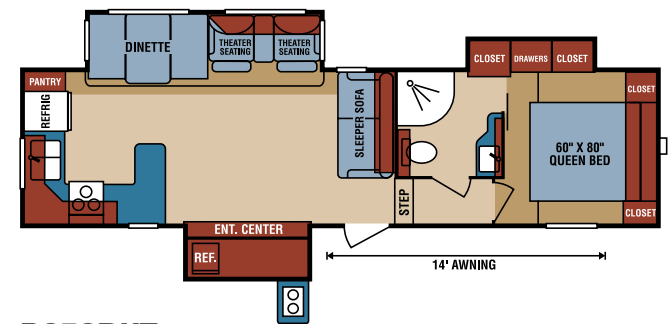
D256RKT UVW TBD • Dry Hitch Wt. TBD NCC TBD • GVWR TBD • Length 33' 9"
