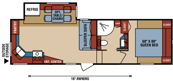
D250RKS UVW 7,620 • Dry Hitch Wt. 1,440 NCC 2,380 • GVWR 10,000 • Length 30' 2"
