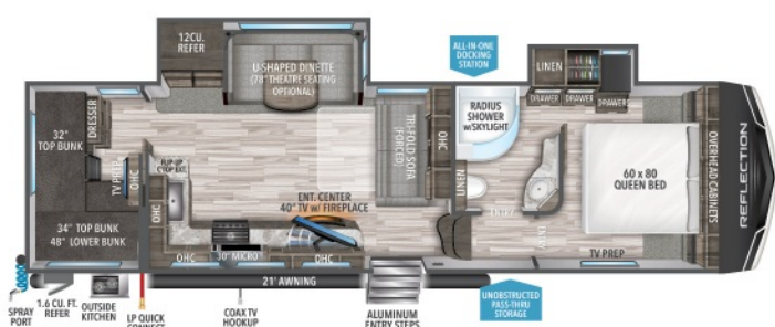
28BH UVW 1 8,997 HITCH 1 1,592 LENGTH 2 34' 8" HEIGHT 3 12' 3" CAPACITY 60 86 43
