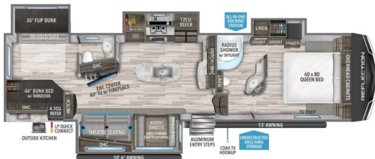
311BHS UVW 1 11,185 HITCH 1 2,180 LENGTH 2 36' 10" HEIGHT 3 12' 3" CAPACITY 60 87 87
