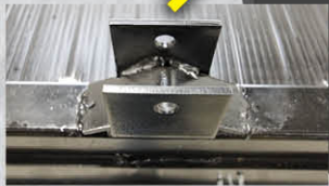
SPRING HANGERS with V-Bracket Reinforcement
