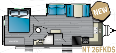
NT 26FKDS LENGTH - 29' 8 1/4" | HEIGHT - 11' 4" | HITCH - 972 LBS. DRY - 6,672 LBS. | GVWR - 9,772 LBS. | SLEEP CAPACITY - 5-6
