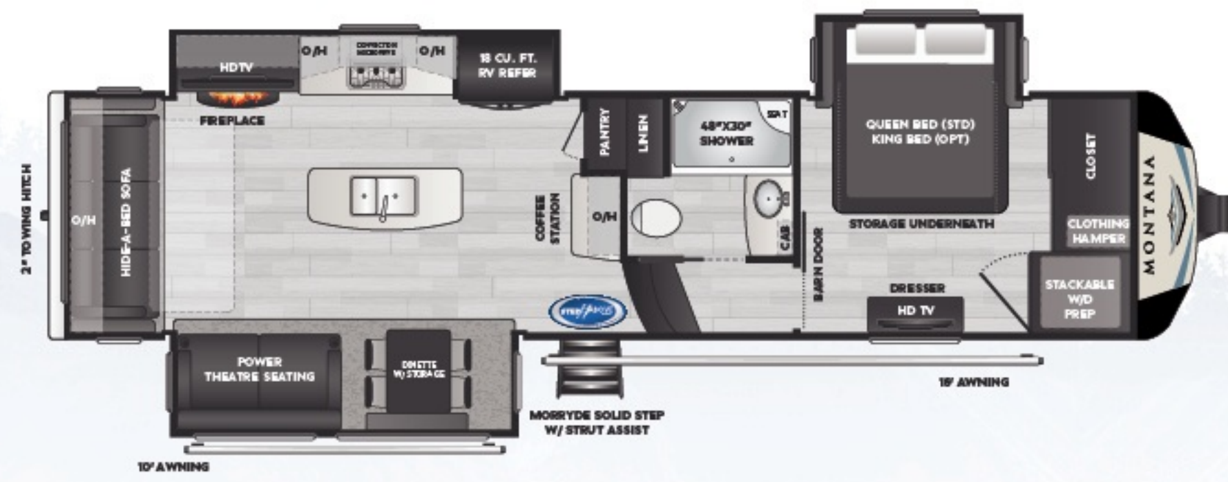
3120/3121RL | Rear living room, three slides RV REFRIGERATOR RES. REFRIGERATOR WEIGHT:12056 LENGTH:35'
