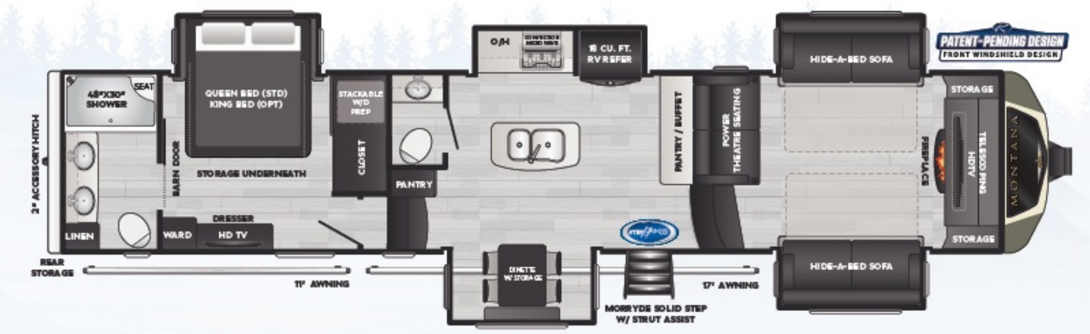
3760/3761FL | Front living, five slides, 1 1/2 baths RV REFRIGERATOR RES. REFRIGERATOR WEIGHT:14147 LENGTH:41'
