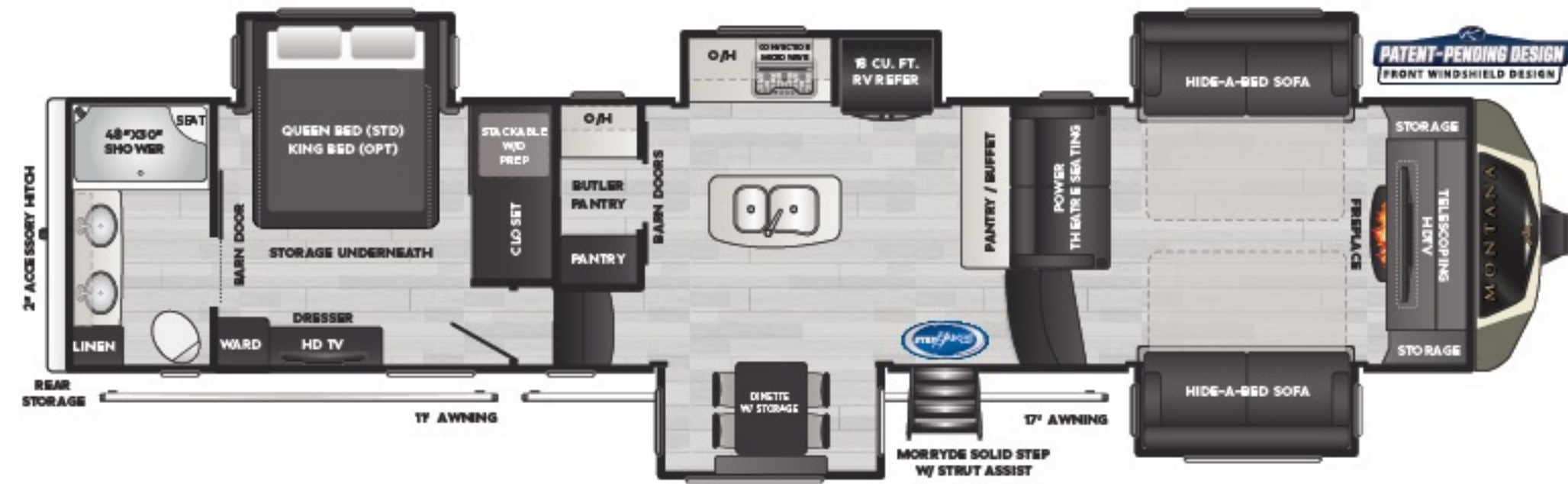
NEW! 3762/3763BP | Front living w/ butler's pantry, five slides RV REFRIGERATOR RES. REFRIGERATOR WEIGHT:14065 LENGTH:41'
